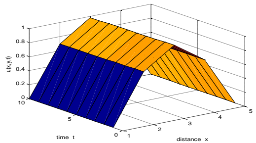
Figure 3: CN-DF-LF solution for the 2-D heat equation at y = 0.5
