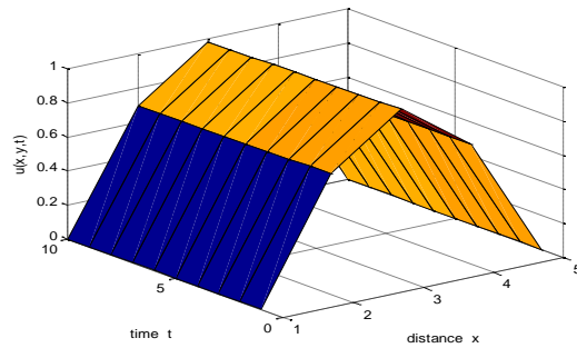
Figure 2: CN solution for the 2-D heat equation when y = 0.5
